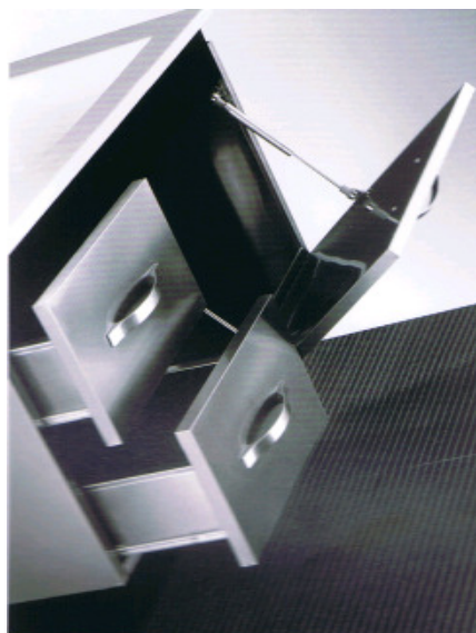
FLL-41102-01 1020x400 mm 980x460x420 mm 1000x146x600 mm
